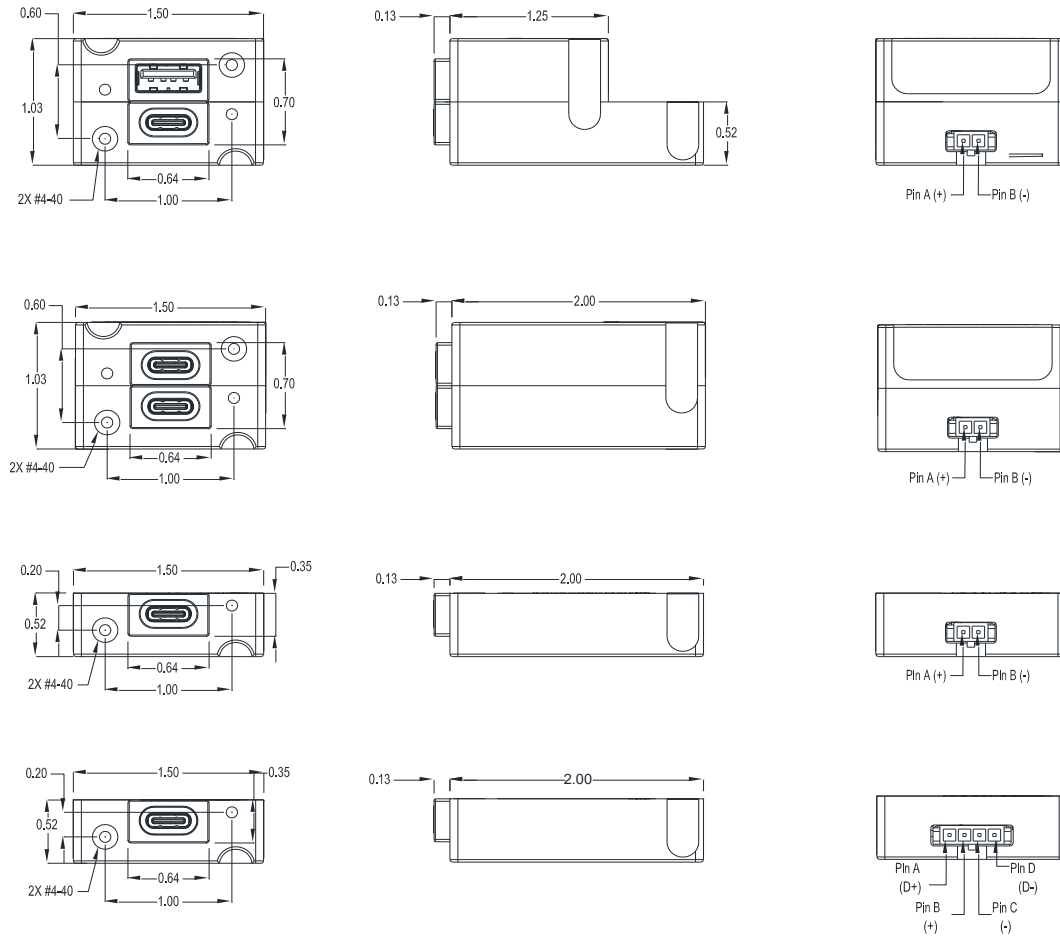
Figure 3.2 TA360 Outline Drawing
