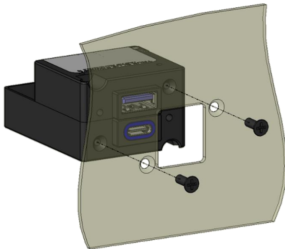
Figure 3.4 Dual Port Rear Mount Installation
