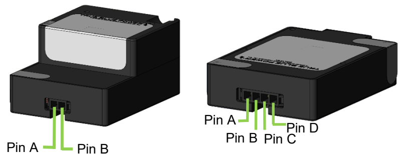
Figure 3.1 Power Input
