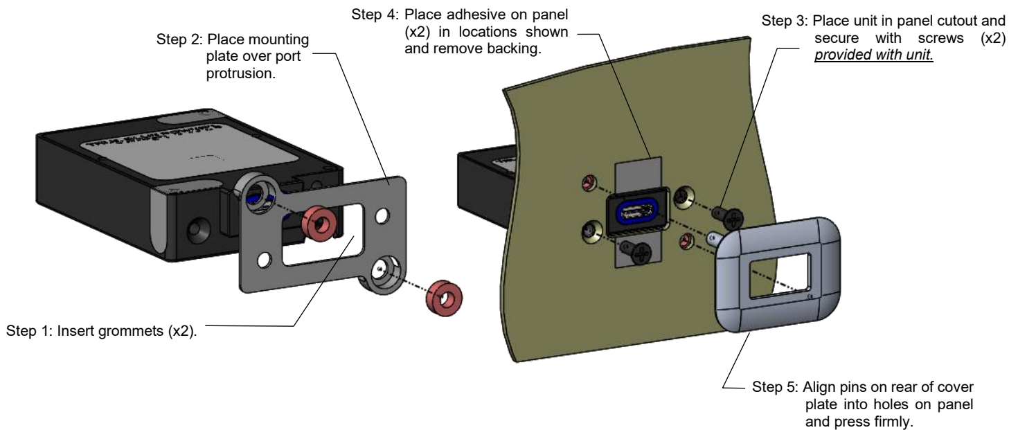
Figure 3.10 Single Port Rear Mount Faceplate Kit
