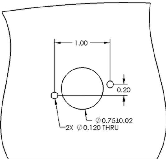
Figure 3.8 Single Port Rear Mount Circular Faceplate
