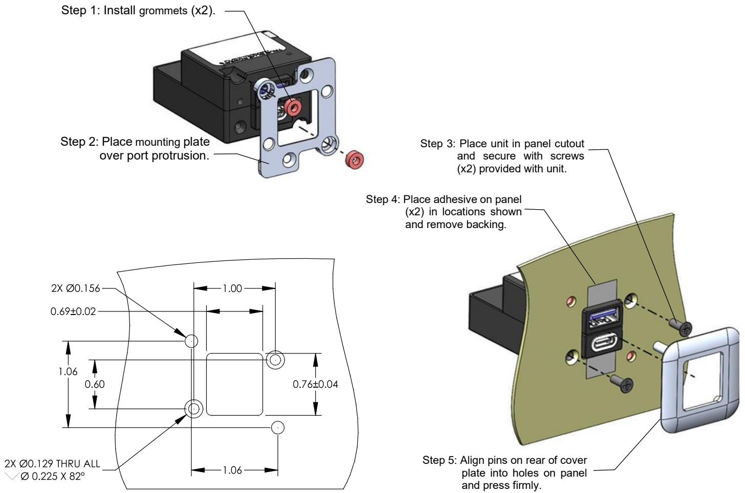
Figure 3.6 Dual Port Rear Mount Faceplate Kit
