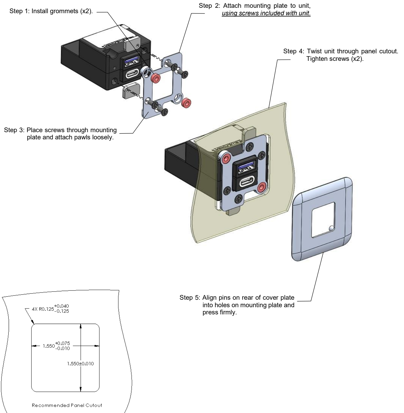
Figure 3.13 Dual Port Front Mount Faceplate Kit
