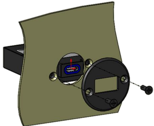
Figure 3.8 Single Port Rear Mount Circular Faceplate
