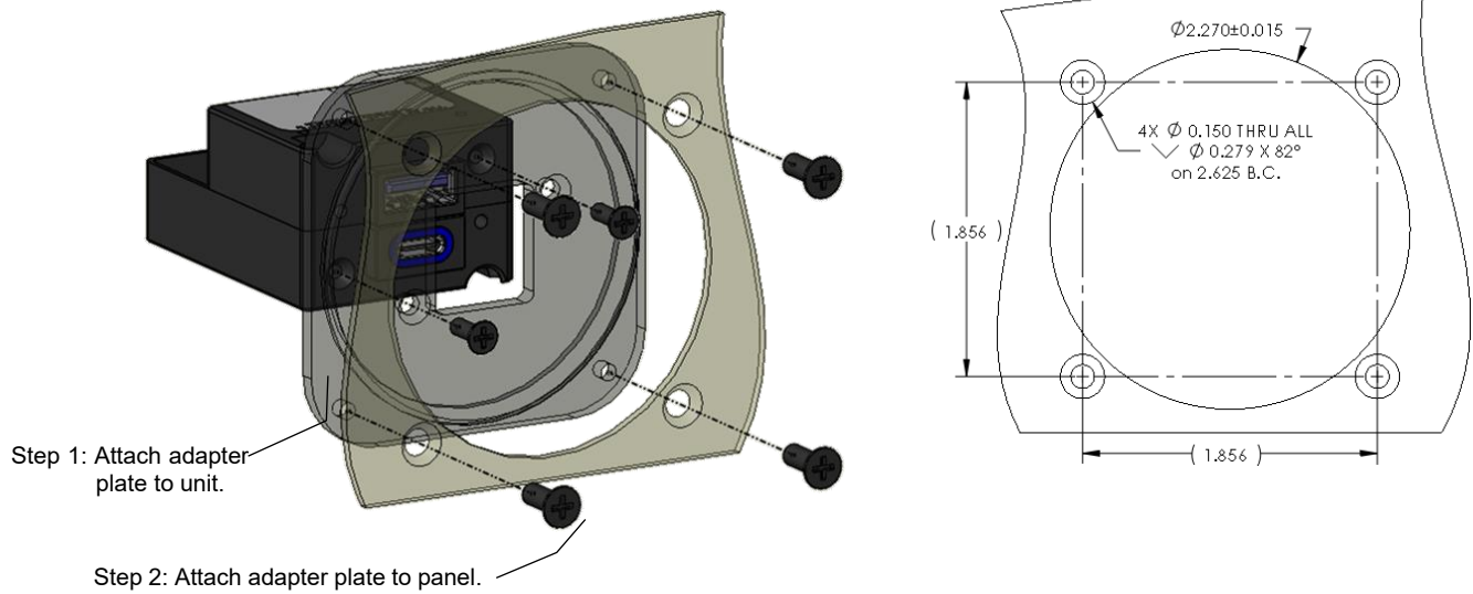
Figure 3.5 Dual Port Instrument Mount Adapter Kit
