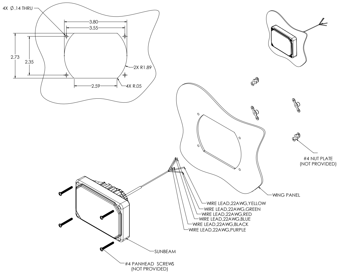
Figure 1. Mounting Diagram
