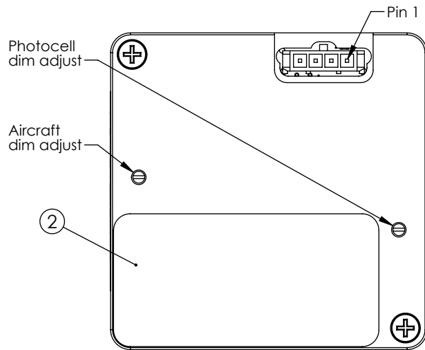
Type 1 configurations
