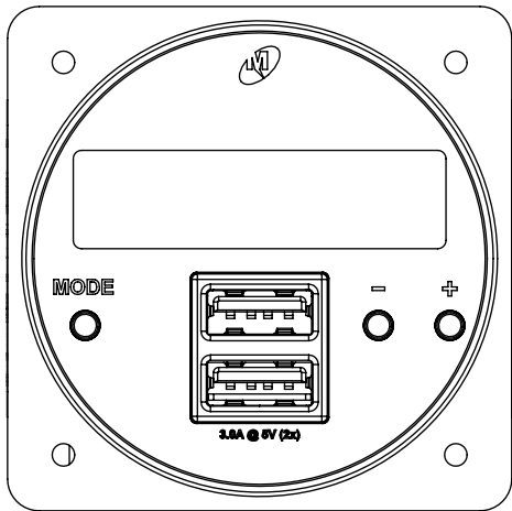
-2 configuration
