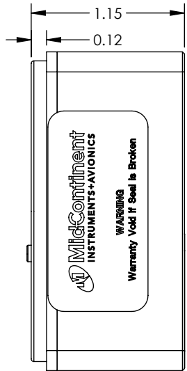
Type 1 configurations
