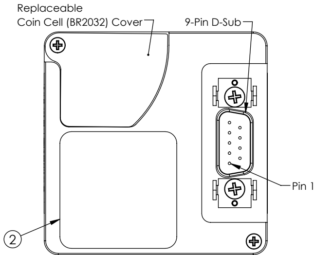
Type 2 configurations
