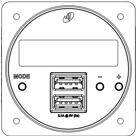
-1 configuration
