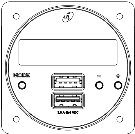
-4 configuration
